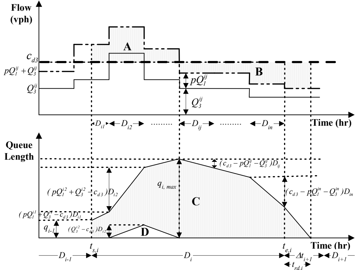
Figure 5.1 Queuing Delay and Dissipation of Queue Length along Detour
