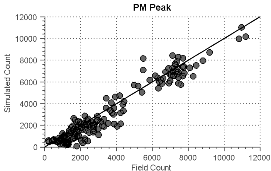
Figure 39. Scatterplot of Field and Simulated P.M. Counts after Calibration.
