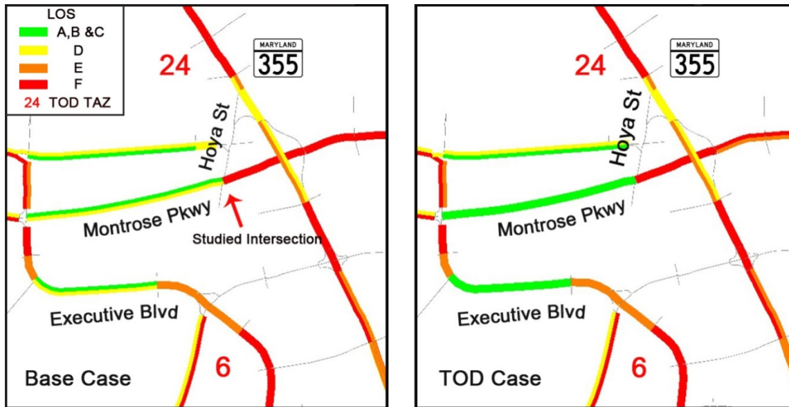
Figure 40. Level of Service (LOS) 4 of the Network around TOD Zones 6 and 24.
