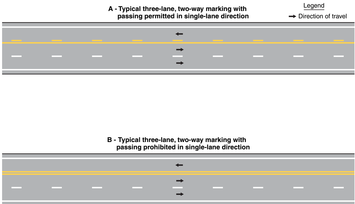
Figure 3B-3. Examples of Three-Lane, Two-Way Marking Applications
