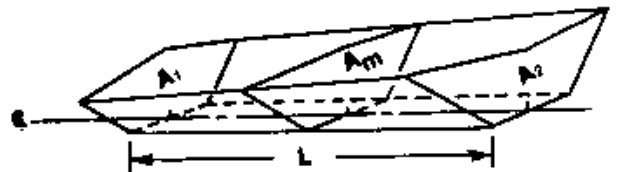
The area of A_m is calculated by using formula 7ai., above. The values used for d , h , b , h' , and h'' are derived by averaging the corresponding values of end sections A_1 and A_2 .
