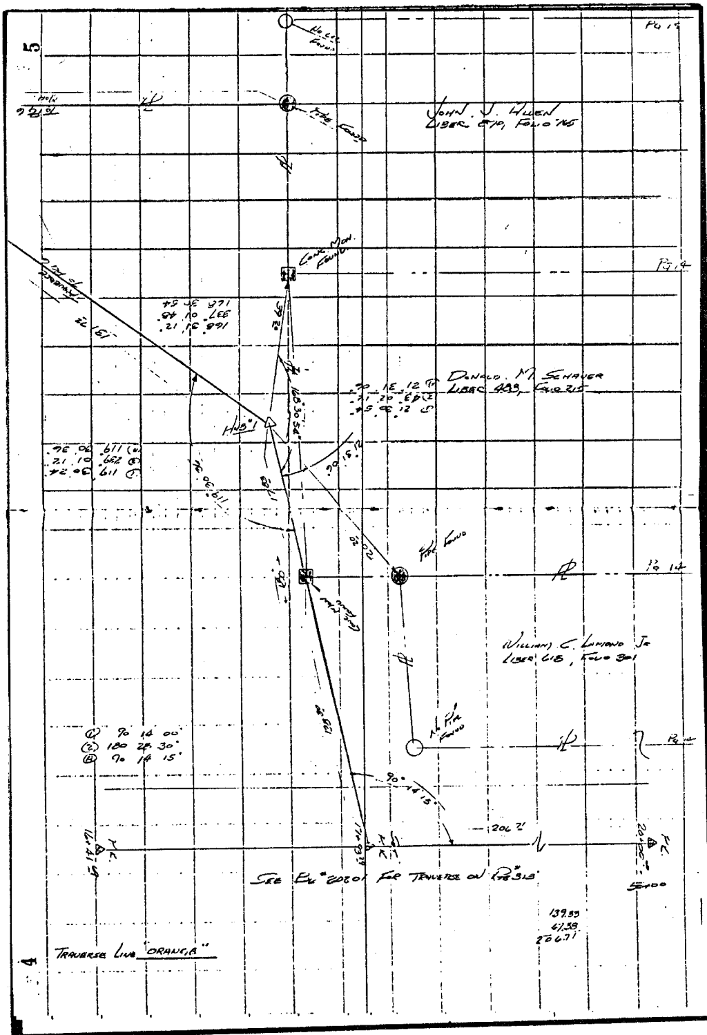
FIGURE 6-05-A(1) SAMPLE METES AND BOUNDS NOTES
