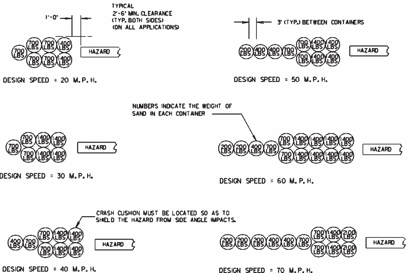
Figure D-92-2TS-1
