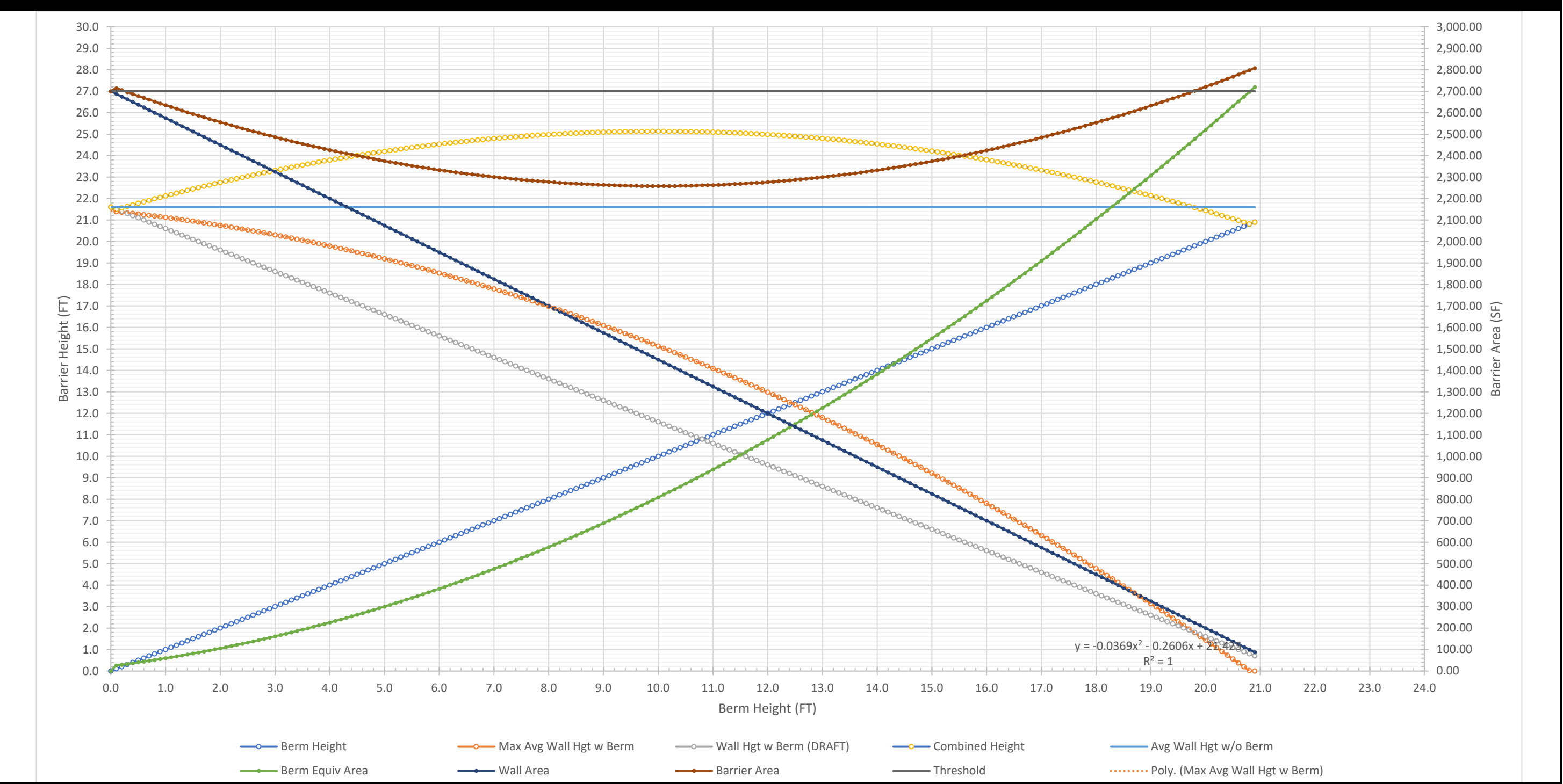
Chart G.2 Barrier Heights and Areas for Walls, Berms, Berm-Wall Combinations using 2:1 side slopes, 125 LF of Frontage, and the 2700 SF-p-r Threshold
