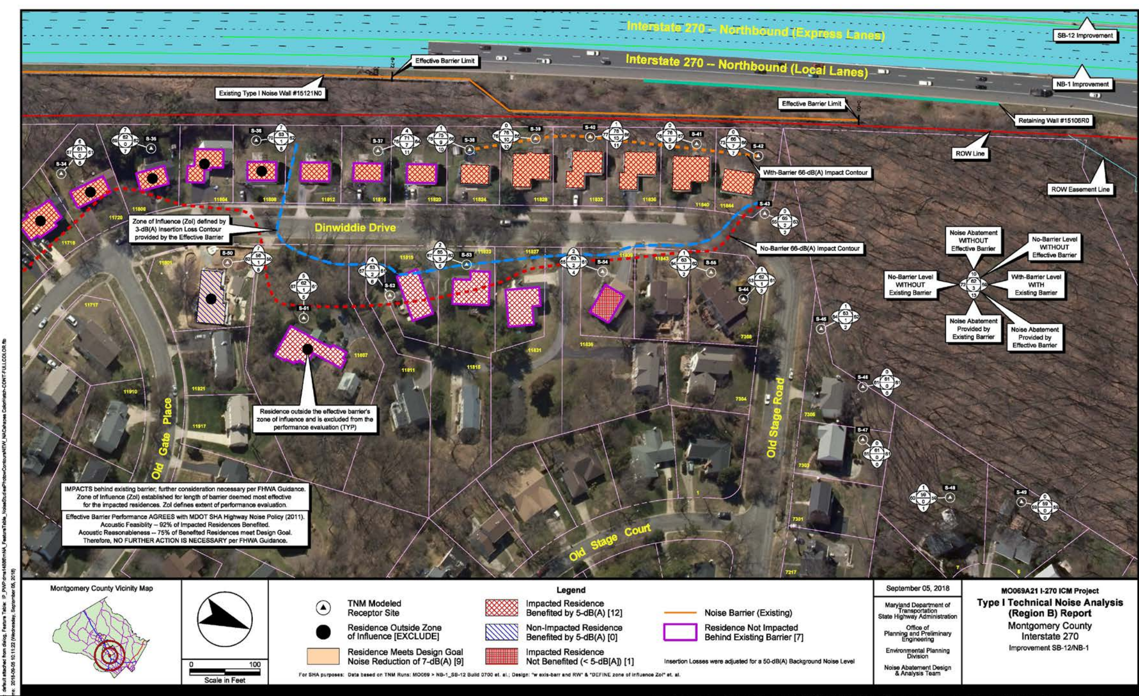
Figure H.1 Effective Barrier Zone of Influence Map for Example H.1
