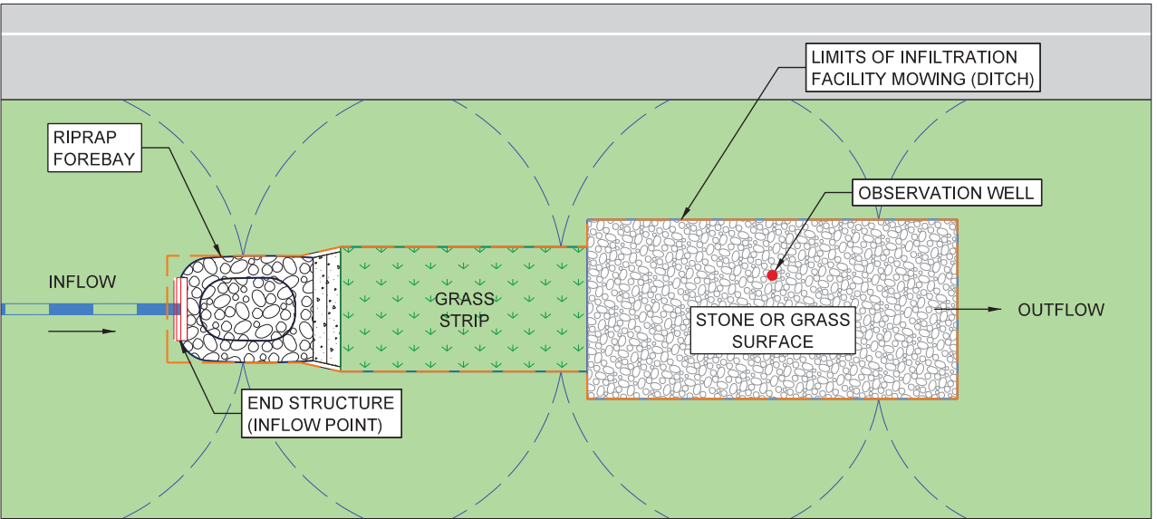
SAMPLE INFILTRATION FACILITY SCHEMATIC
