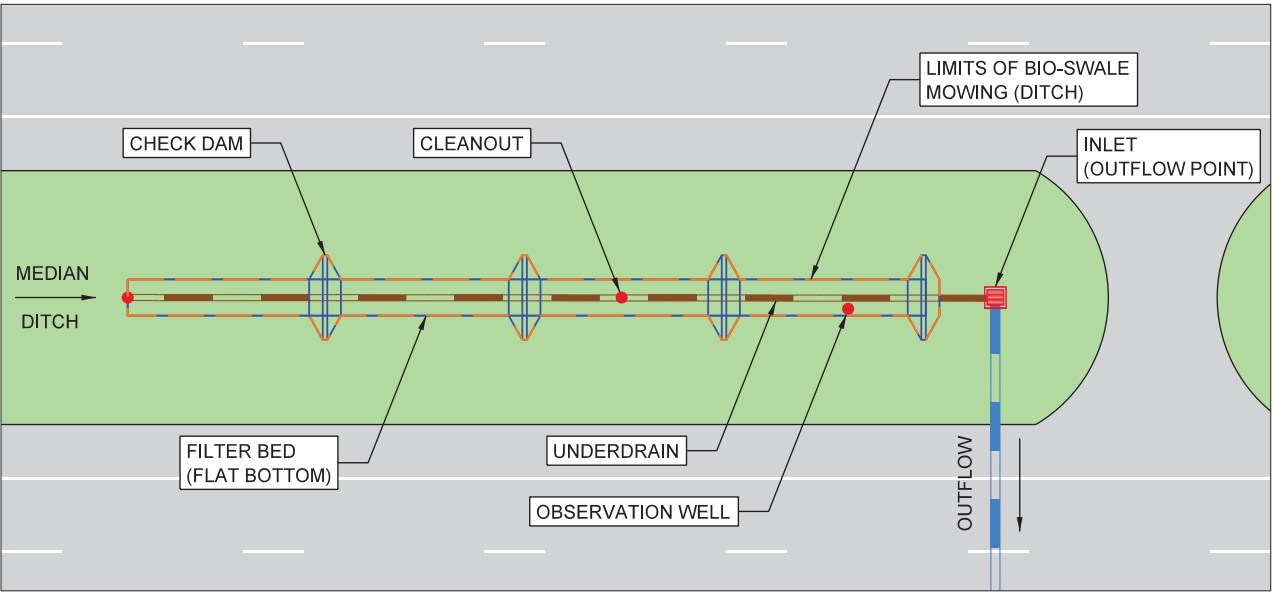
SAMPLE BIO-SWALE SCHEMATIC
