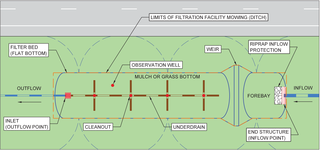
SAMPLE FILTRATION FACILITY SCHEMATIC
