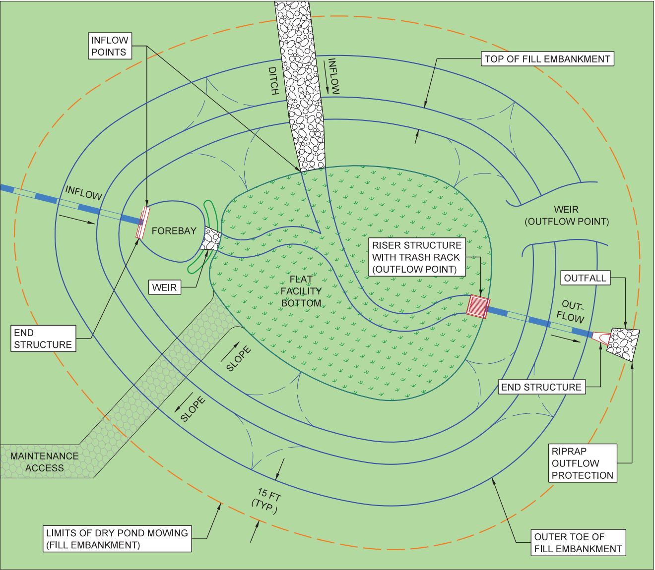
SAMPLE DRY POND SCHEMATIC
