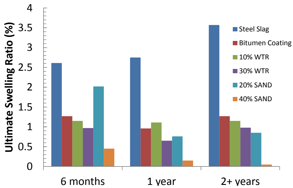
Figure 5.1. Effect of treatment methods on the ultimate swelling ratio
