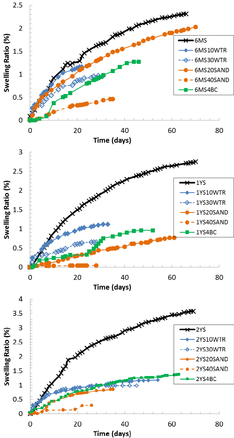
Figure 2.5 Swelling curves for of pure, bitumen-coated, and WTR or sand-amended steel slag aged for (a) 6 months, (b) 1 year, and (c) 2 years. (Note: S: steel slag, BC: bituminous coating, WTR: water treatment residual)
