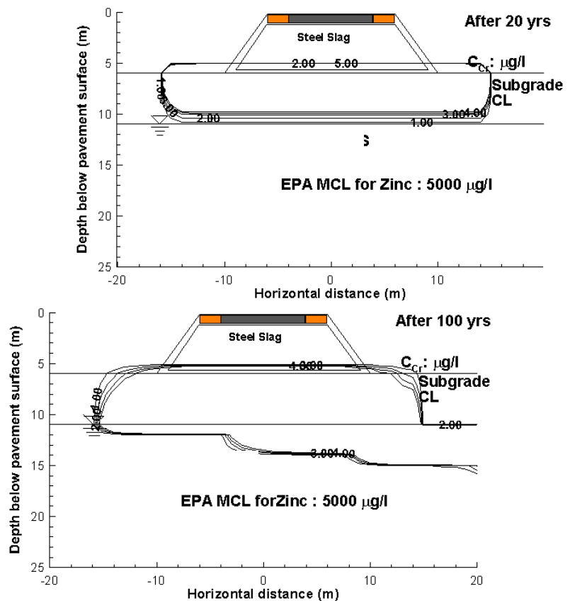
Figure 4.11. Predicted Zn concentrations in vadose zone and groundwater for simulating flow of S leachate through subgrade CL.
