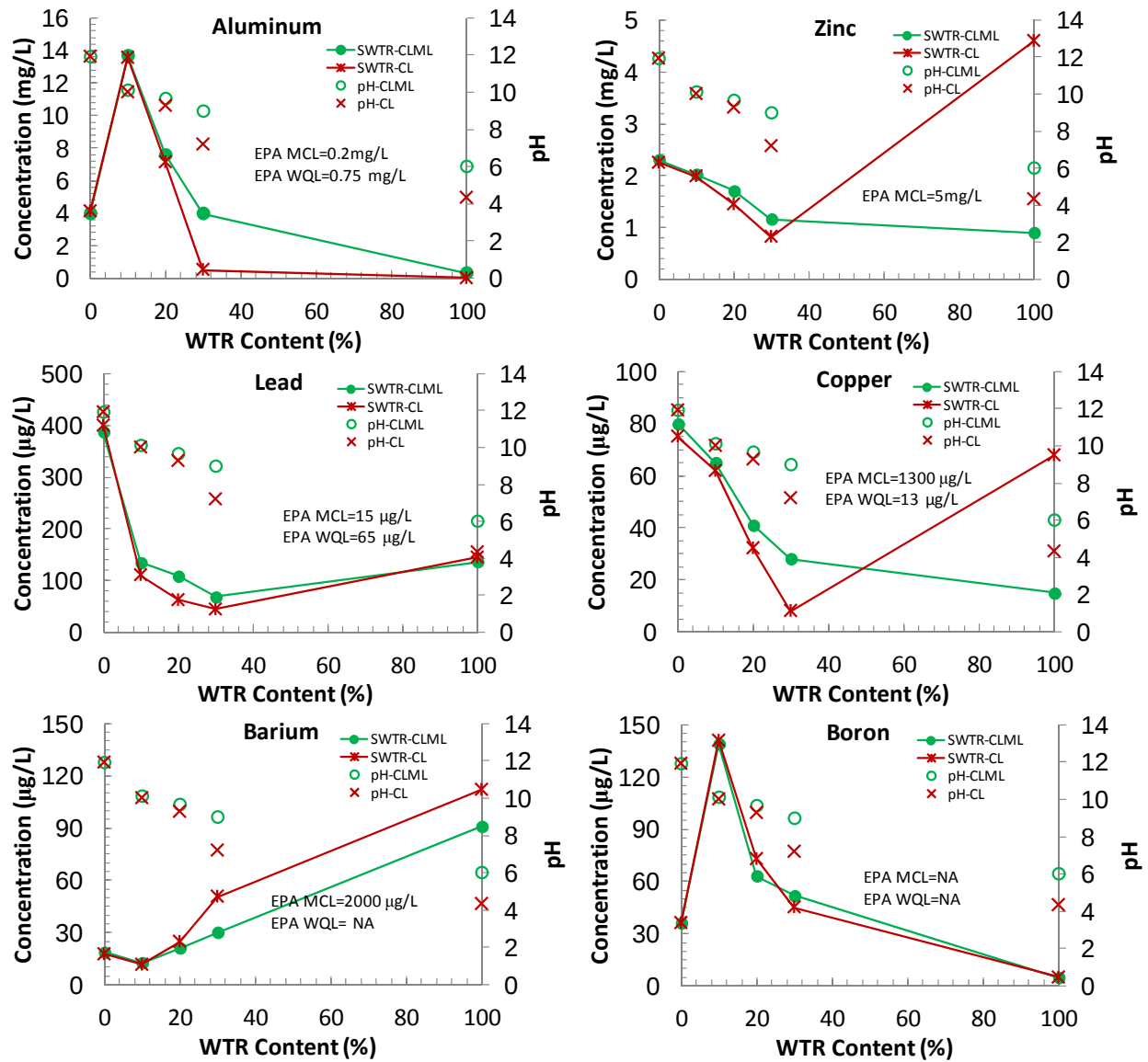
Figure 4.5. Effect of WTR content on WLT concentrations of a) aluminum, b) zinc, c) lead, d) copper, e) barium and f) boron. Leachates of mixtures prepared with 10%, 20% and 30% steel slag are run for another 18 hours with subgrade. 0% and 100% WTR content corresponds to steel slag only and WTR only specimens, respectively.
