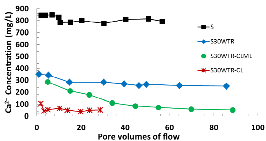
Figure 4.7 Elution curves for \text{Ca}^{2+}
