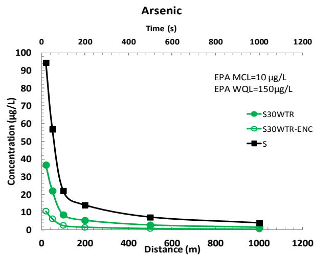
Figure 3.9. Surface water concentrations of a) aluminum, b) chromium, c) arsenic with increasing horizontal distance.
