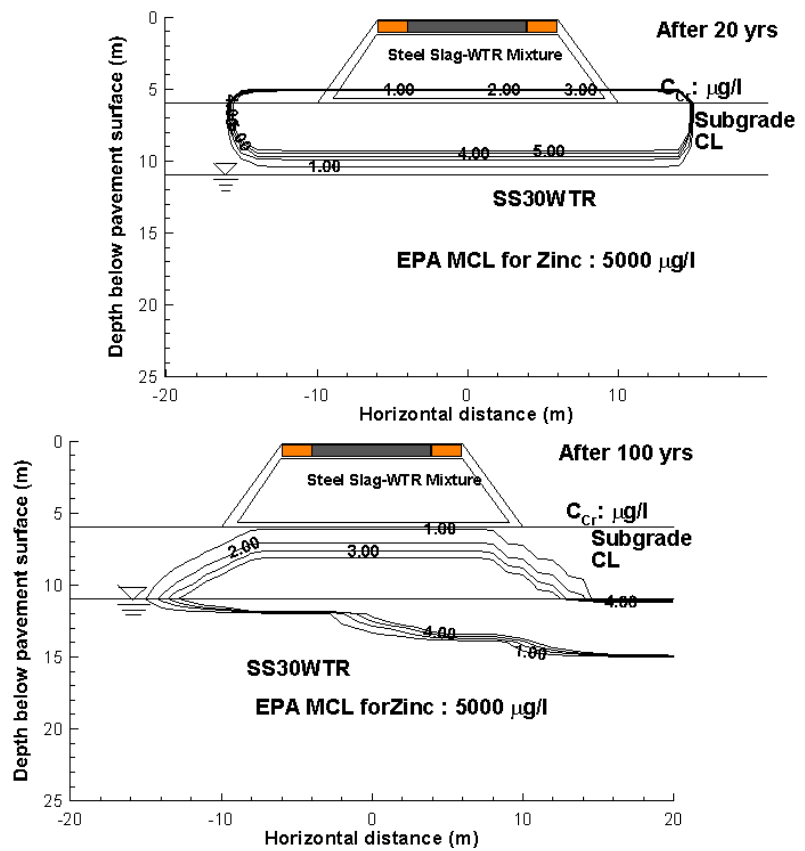
Figure 4.9. Predicted Zn concentrations in vadose zone and groundwater for simulating flow of S30WTR leachate through subgrade CL.
