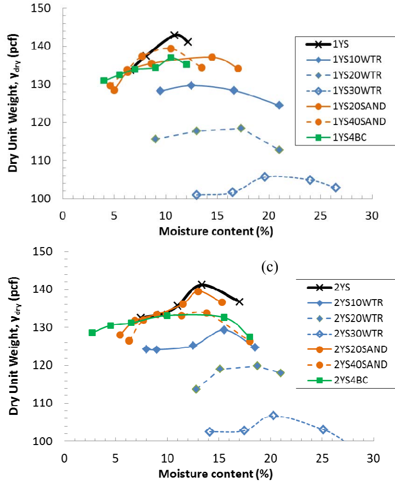
Figure 2.4 Compaction curves of pure, bitumen-coated and WTR or sand-amended steel Slag, aged for (a) 6 months, (b) 1 year and (c) 2 years (Note: S: steel slag, BC: bituminous coating, WTR: water treatment residual).
