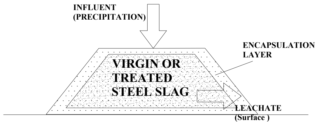
Figure 3.3. Conceptual model to analyze the flow of steel slag into surface waters.
