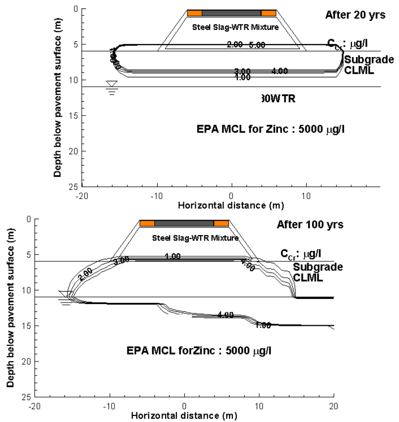
Figure 4.10. Predicted Zn concentrations in vadose zone and groundwater for simulating flow of S30WTR leachate through subgrade CLML.
