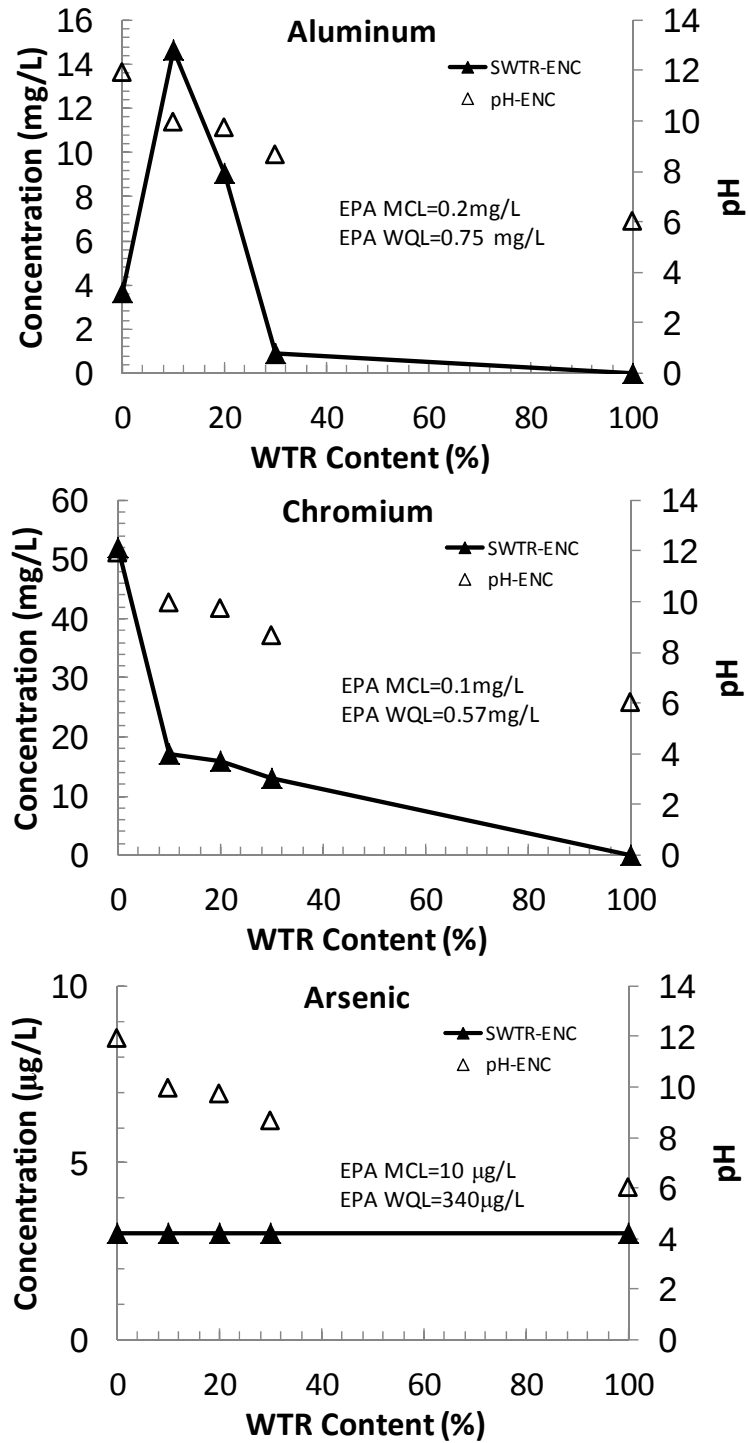
Figure 3.5. Effect of WTR content on sequential water leach test concentrations of a) aluminum (Al), b) chromium (Cr), and c) arsenic (As). 0% and 100% WTR content corresponds to pure SS and pure WTR specimens, respectively.
