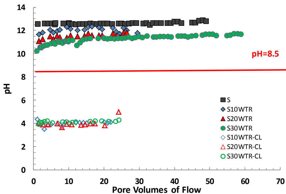
Figure 4.6. Effluent pH in CLTs on (a) CL-ML soil, and (b) CL soil
