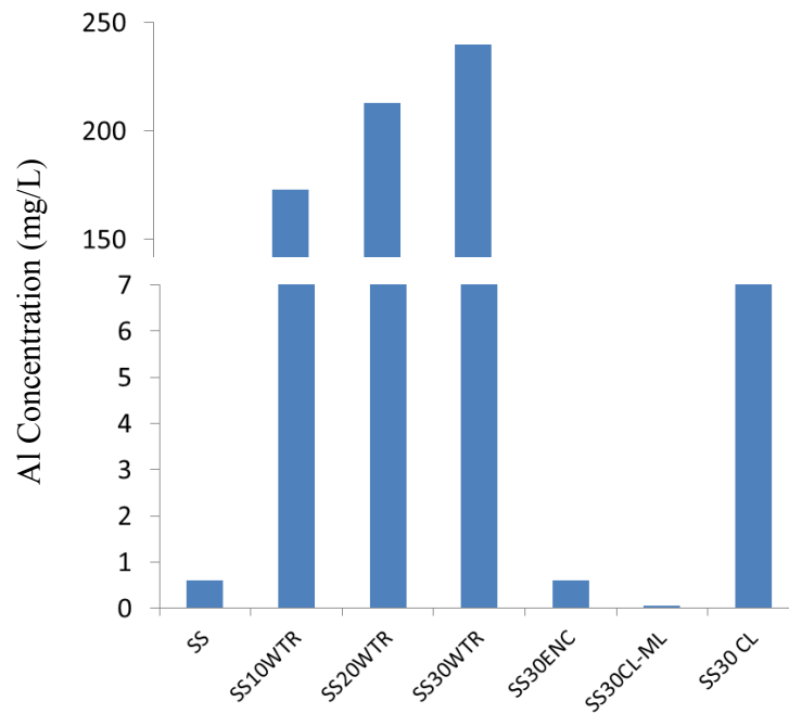
Figure 5.3. Effect of subgrade type on Al-concentrations
