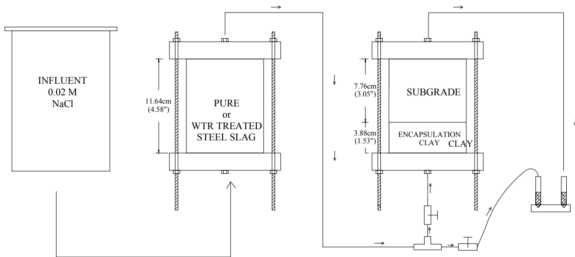
Figure 4.2. Sequential Column Leach Test (SCLT) setup
