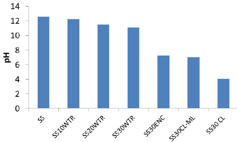
Figure 5.2. Effect of subgrade type on effluent pH
