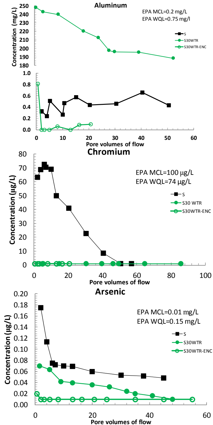
Figure 3.8. CLT elution curves for a) aluminum, b) chromium, c) arsenic.
