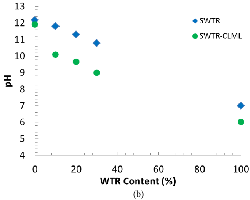
Figure 4.4. Effect of WTR content and flow through subgrade on pH of the leachates past through (a) CL soil, and (b) CL-ML soil. Note: SWTR designate the specimens prepared with different WTR percentages whereas SWTR-CL and SWTR-CLML designate specimens that are prepared by mixing effluent leachates from the SWTR mixtures with subgrade CL and CLML, respectively.
