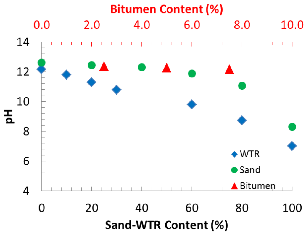
Figure 3.1. Results of preliminary batch water leach tests
