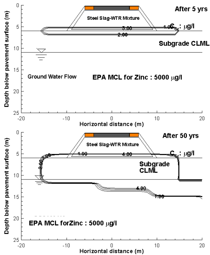
Figure 4.10. Predicted Zn concentrations in vadose zone and groundwater for simulating flow of S30WTR leachate through subgrade CLML.
