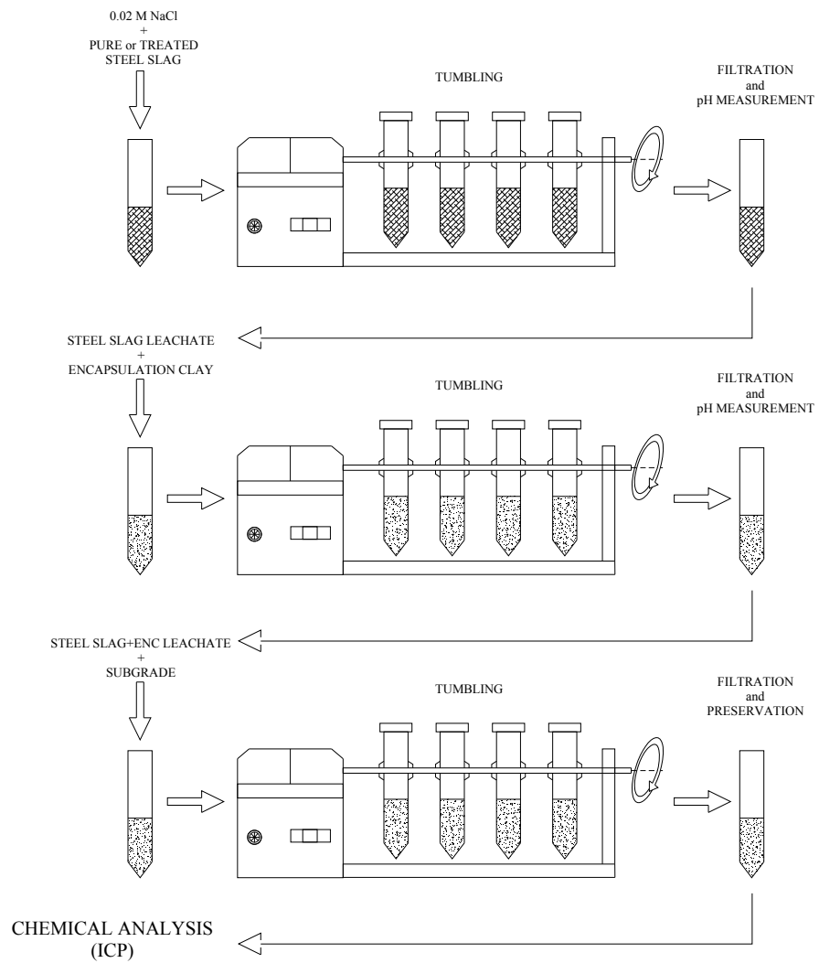
Figure 4.1. Sequential Water Leach Test (SWLT) setup
