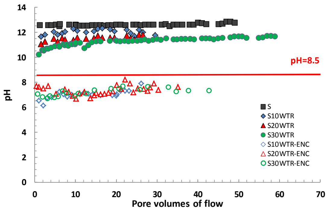
Figure 3.6. Effluent pH in CLTs.
