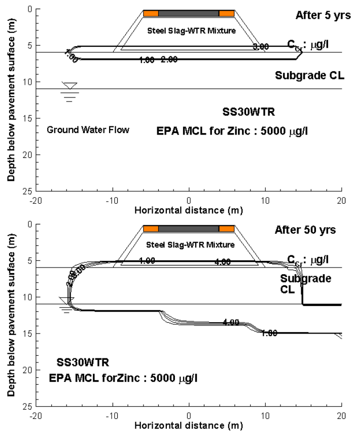
Figure 4.9. Predicted Zn concentrations in vadose zone and groundwater for simulating flow of S30WTR leachate through subgrade CL.
