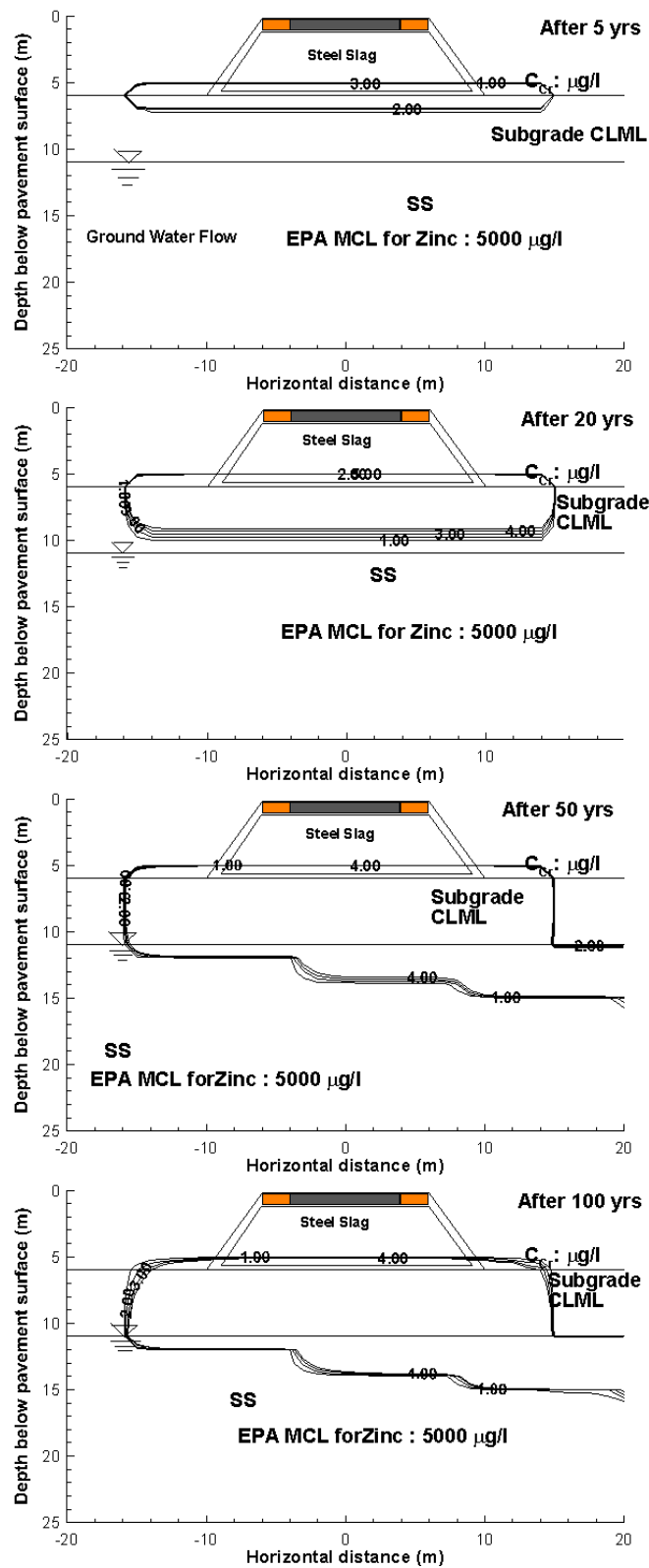
Figure 4.12. Predicted Zn concentrations in vadose zone and groundwater for simulating flow of S leachate through subgrade CLML
