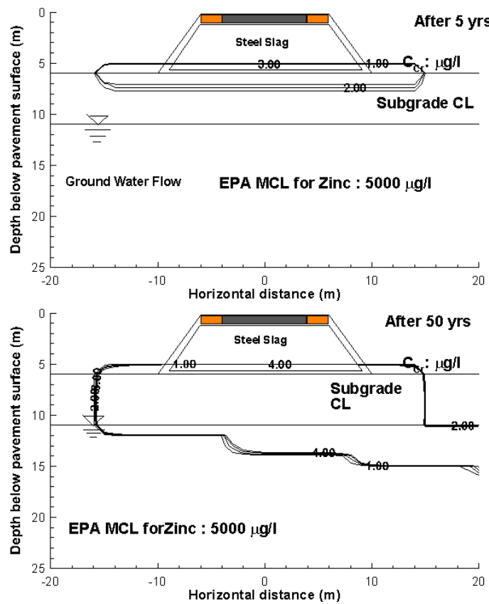
Figure 4.11. Predicted Zn concentrations in vadose zone and groundwater for simulating flow of S leachate through subgrade CL.
