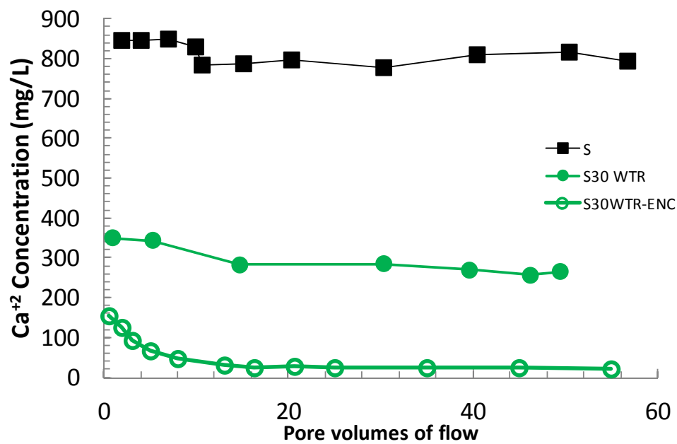
Figure 3.7. Elution curves for \text{Ca}^{2+} .
