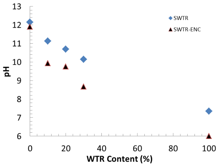
Figure 3.4. Effect of WTR content and presence of encapsulation clay on pH of the slag mixtures. Note: SWTR designate the specimens prepared with different WTR percentages whereas SWTR-ENC designates specimens that are prepared by mixing encapsulation clay and effluent leachates from SWTR mixtures.
