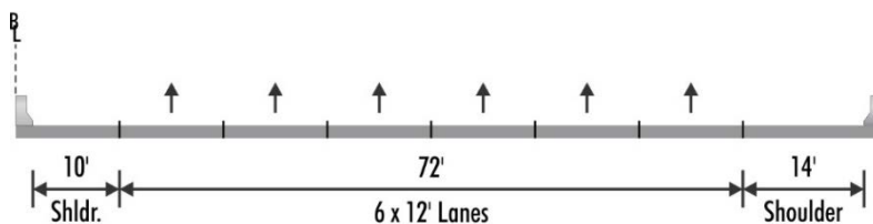
Figure C-6. Southbound 12 Typical Sections – I-270 from Montrose Road to West Spur
