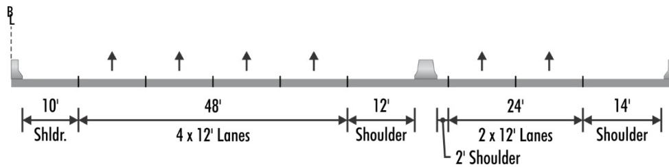
NB 1 EXISTING – I-270 Express Lanes
