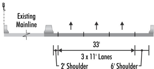
SB 6 PROPOSED – I-270 Local Lanes
