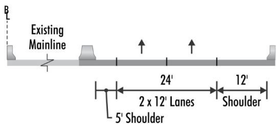
SB 6 EXISTING – I-270 Local Lanes
