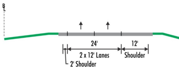
Figure C-15. Northbound 5 Typical Sections – I-270 Mainline
