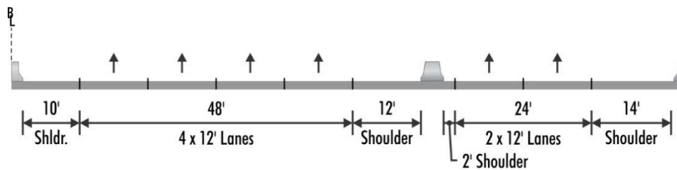
Figure C-5. Southbound 12 Typical Sections – I-270 Express Lanes
