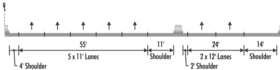
NB 1 PROPOSED – I-270 Express Lanes
