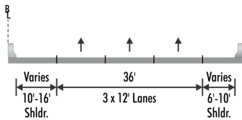
Figure C-7. Southbound 12 Typical Sections – I-270 West Spur
